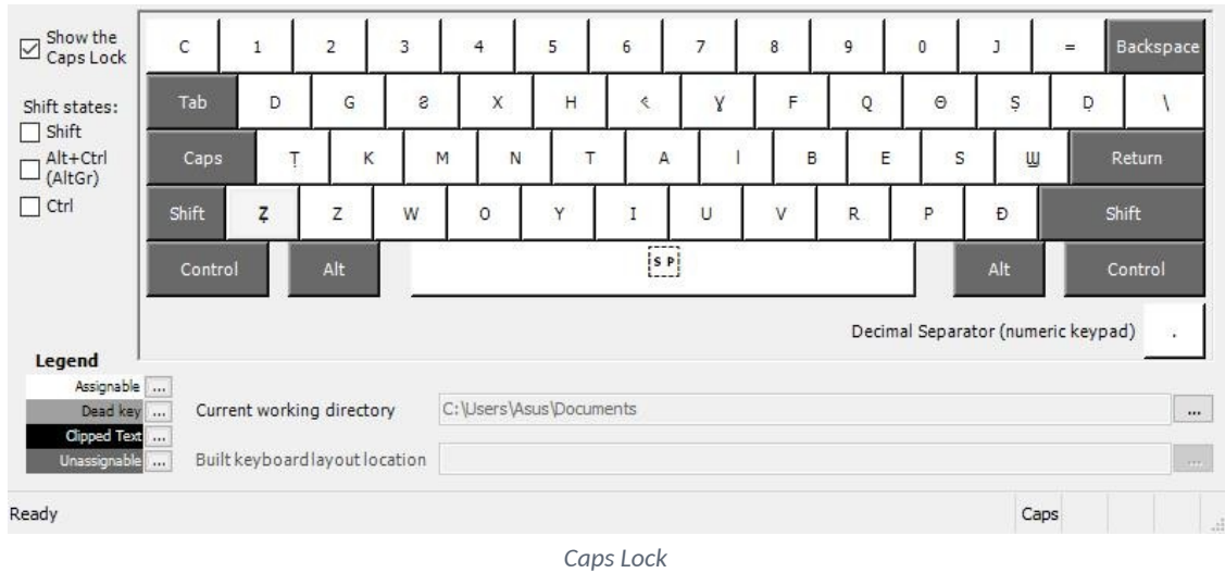
Caps Lock
